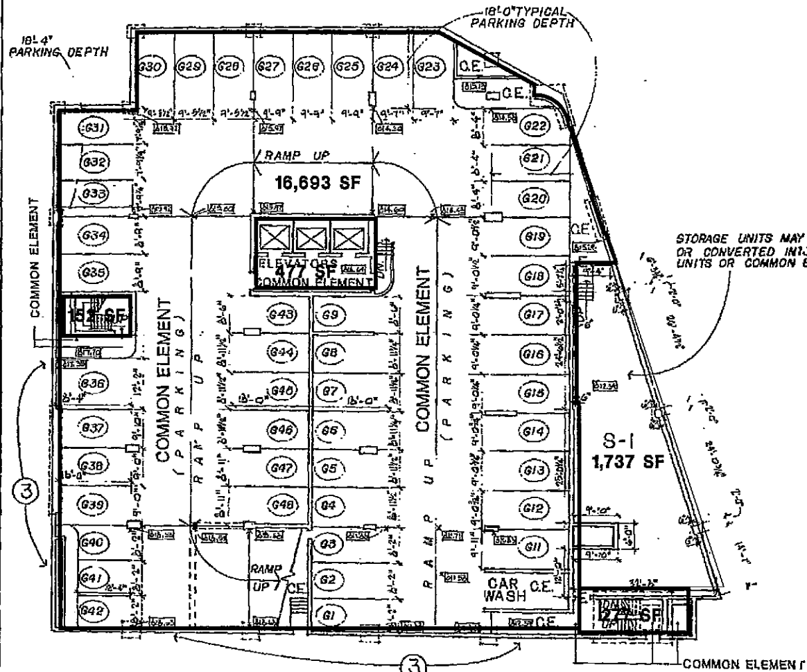
G-1 FLOOR PLAN
